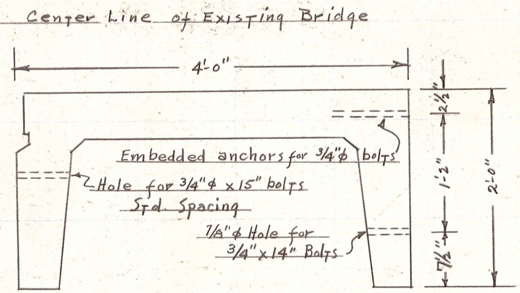
SECTION THRU OUTSIDE SLAB Scale 1" = 1'-0"
