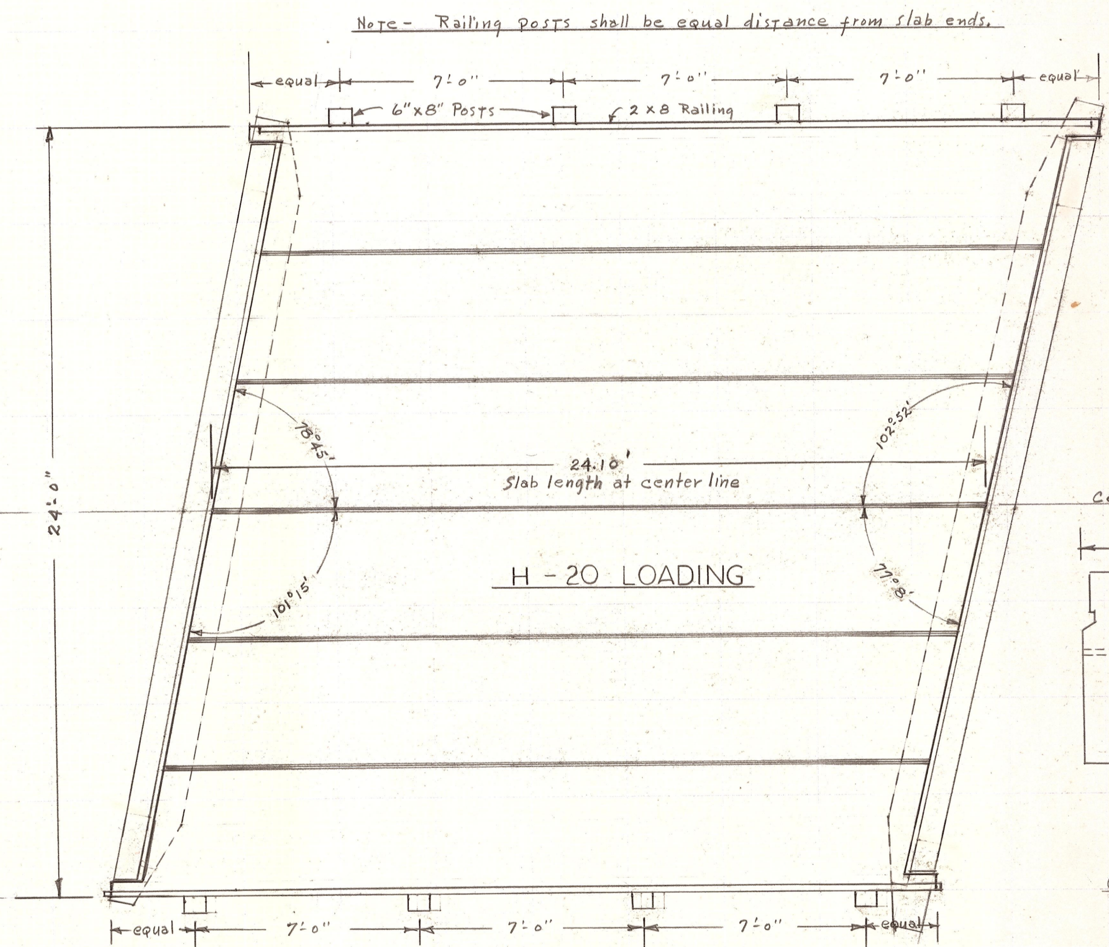
PLAN Scale 1" = 3'-0"
